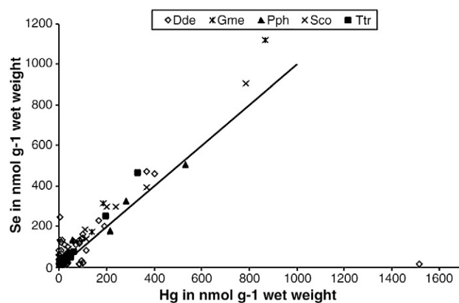
Fig. 4. Molar Se and molar Hg concentrations ( \text{nmol g}^{-1} wet weight) in liver tissue of Dde: common dolphin ( Delphinus delphis ), Gme: pilot whale ( Globicephala melas ), Pph: harbour porpoise ( Phocoena phocoena ), Sco: striped dolphin ( Stenella coeruleoalba ) and Ttr: bottlenose dolphin ( Tursiops truncatus ) from the North West Iberian Peninsula. The solid line indicate the Hg:Se molar ratio of 1.
