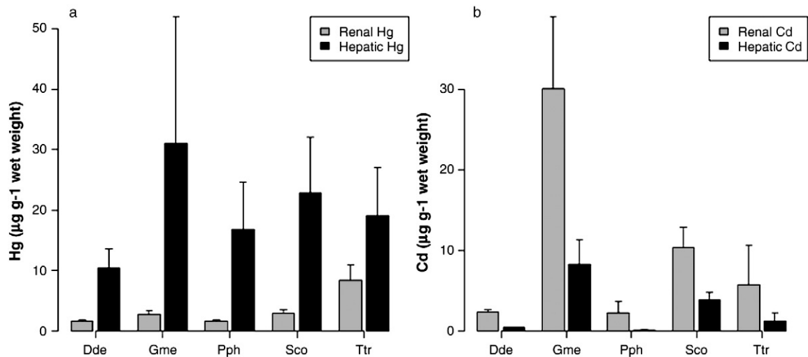
Fig. 2. Concentrations (mean \pm SE, standard error, in \mu\text{g g}^{-1} wet weight) of mercury (a) and cadmium (b) in the liver and kidney of Dde: common dolphin ( Delphinus delphis ), Gme: pilot whale ( Globicephala melas ), Pph: harbour porpoise ( Phocoena phocoena ), Sco: striped dolphin ( Stenella coeruleoalba ) and Ttr: bottlenose dolphin ( Tursiops truncatus ) from the North West Iberian Peninsula. Mercury (Hg) and cadmium (Cd) were chosen since each of them represented one of the two patterns of tissue distribution of the 14 trace elements analysed.
