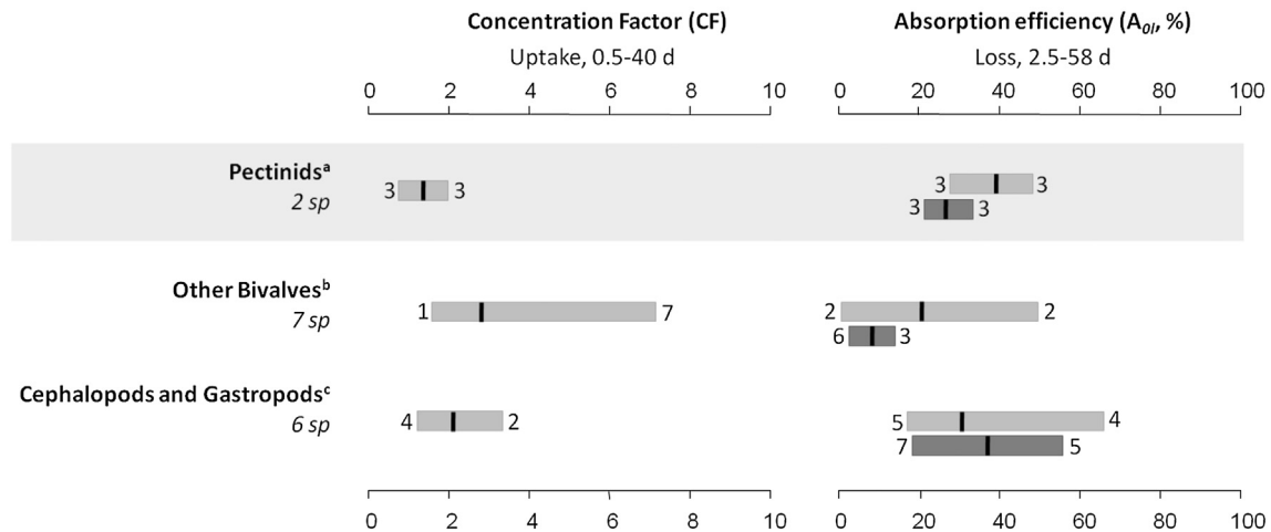
Fig. 2. Comparison of concentration factors (CF) and percentages of long-term component absorption efficiency ( A_{0t} ) for different taxa of molluscs in experimental conditions. Values are mean \pm SD. When the values were not directly available, a graphical estimate was performed from uptake and depuration kinetics. Bars are ranges of values. Light grey and dark grey bars represent respectively seawater and food pathways. Black vertical lines indicate means calculated from all the considered values. The numbers next to grey bars represent the number of values below and above the calculated means. a Present study and Metian et al. (2011), b (Ueda et al., 1978; Nolan and Dahlgaard, 1991; Hutchins et al., 1998; Ke et al., 2000; Wang et al., 2000; Güngör et al., 2001; Qureshi et al., 2007; Kalaycı et al., 2013), c (Bryan, 1963; Bustamante et al., 2006; Lacoue-Labarthe et al., 2010).
