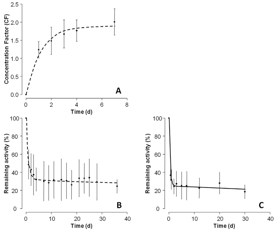
Fig. 1. (A) Uptake kinetics of ^{134}\text{Cs} in M. varia exposed for 7 d to dissolved radiotracers ( n = 9 ); (B) subsequent 36-d depuration kinetics ( n = 9 ) and (C) 30-d depuration kinetics after ^{134}\text{Cs} -labeled food ingestion ( n = 6 ). All values are mean \pm SD.
