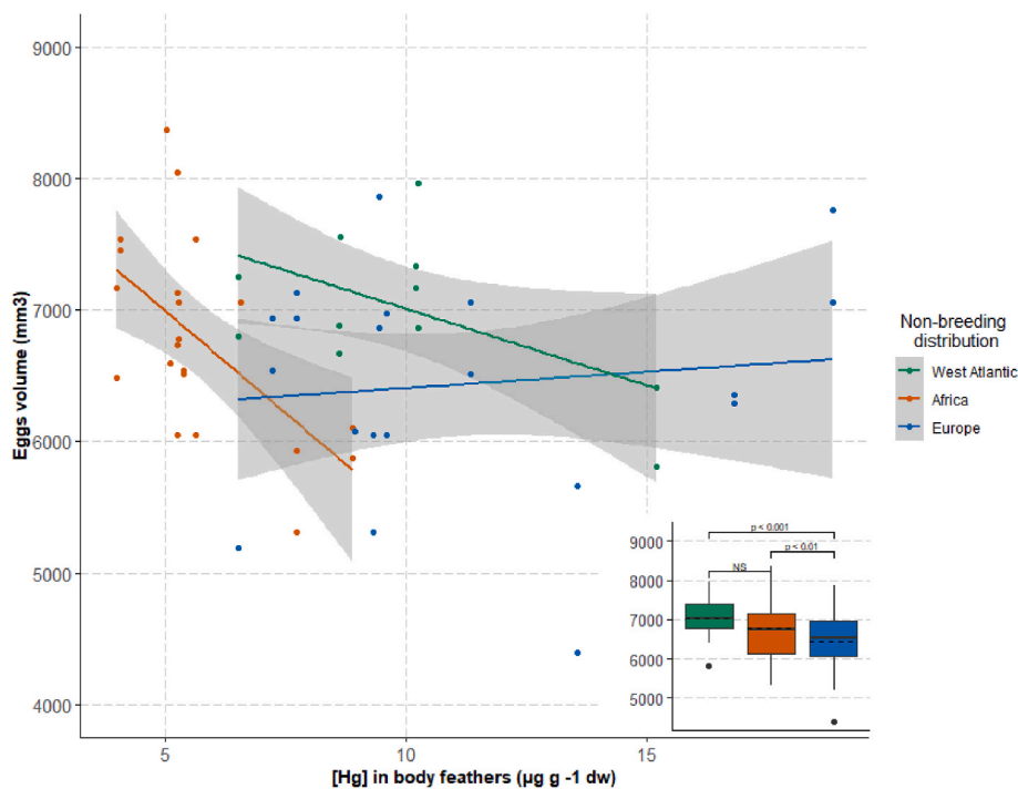
Fig. 3. Egg volume ( \text{mm}^3 ) in relation to Hg concentration ( \mu\text{g g}^{-1} ) in body feathers, depending on female winter distribution. Mean egg volume was 6439 \pm 815 \text{ mm}^3 for females wintering in Europe, 6900 \pm 687 \text{ mm}^3 for female wintering off Africa and 7022 \pm 579 for those wintering in West Atlantic. Egg volume is represented using the same colour code as in Fig. 1. The shaded grey area represents the 95% confidence interval. (For interpretation of the references to colour in this figure legend, the reader is referred to the Web version of this article.)
