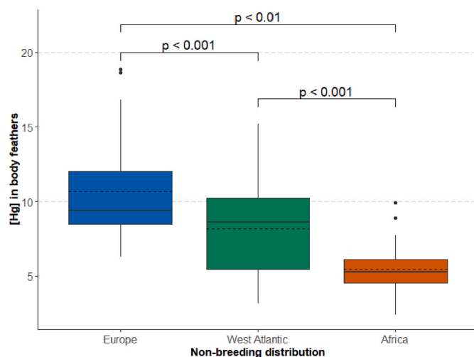
Fig. 2. Mean Hg concentrations ( \mu\text{g g}^{-1} ) measured in body feathers in relation to bird winter distribution. Mean Hg concentrations are represented by dashed black lines and are 10.61 \pm 3.60 \mu\text{g g}^{-1} dw for Europe, 8.37 \pm 3.49 \mu\text{g g}^{-1} dw for West Atlantic and 5.19 \pm 1.91 \mu\text{g g}^{-1} dw for Africa. Boxplots show the median (horizontal black line within the boxes), 1st and 3rd quartiles, the minimum (1st–1.5x interquartile range) and maximum (3rd–1.5x interquartile range) concentrations (lower and upper whiskers) and outliers.
