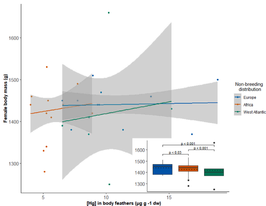
Fig. 4. Female body mass (g) in relation to Hg concentration ( \mu\text{g g}^{-1} ) in body feathers and their winter distribution. Mean values of female body mass were 1443.0 \pm 45.6 \text{ g} for female wintering in Europe, 1420.5 \pm 62.9 \text{ g} for female wintering off Africa and 1418.3 \pm 128.0 \text{ g} for female wintering in West Atlantic. Female body masses are represented using the same colour code as in Fig. 1. The shaded grey area represents the 95% confidence interval. (For interpretation of the references to colour in this figure legend, the reader is referred to the Web version of this article.)
