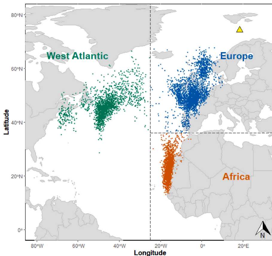
Fig. 1. Winter distribution (November–January) of the tracked great skuas (i.e. both females and males, n = 59 ) breeding in Bjørnøya in winters 2014–2015 to 2016–2017 (yellow triangle) and wintering in Africa (orange), Europe (blue) and West Atlantic (green). Each dot represents daily distribution per individual from November to January (see methods). (For interpretation of the references to colour in this figure legend, the reader is referred to the Web version of this article.)
